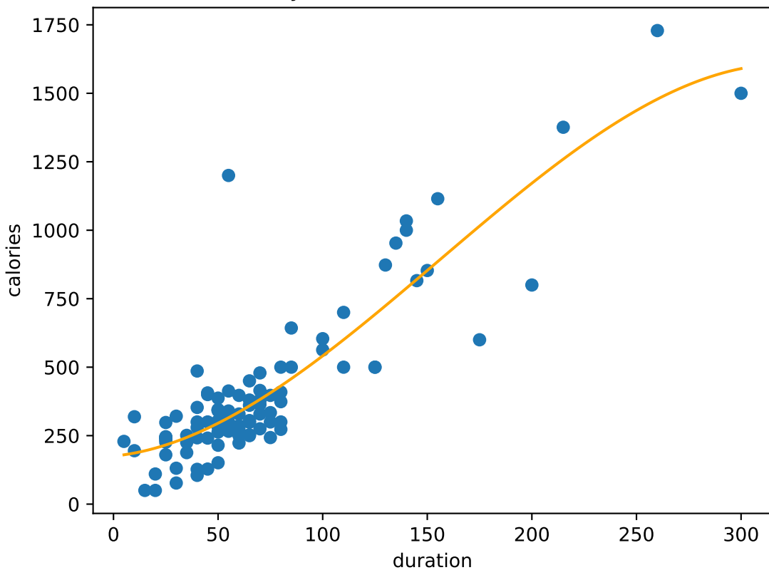
Poly (K=3 duration vs calories)
